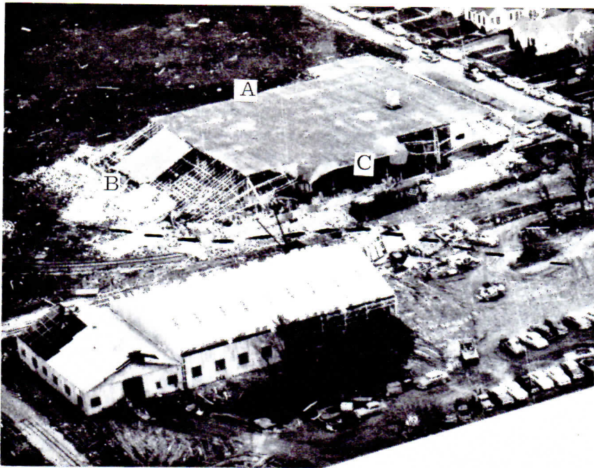
FIGURE 3.—Damage to a building of solid masonry wall construction. Labels A, B, C, refer to walls discussed in text. Dashed line shows approximate path of tornado, moving toward the left.
