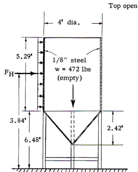
FIGURE 2.—Plan and elevation views of tank, item no. II. Support consists of four legs and four horizontal braces. All are 1\frac{1}{2} by 1\frac{1}{2} by \frac{3}{16} -inch angles.
