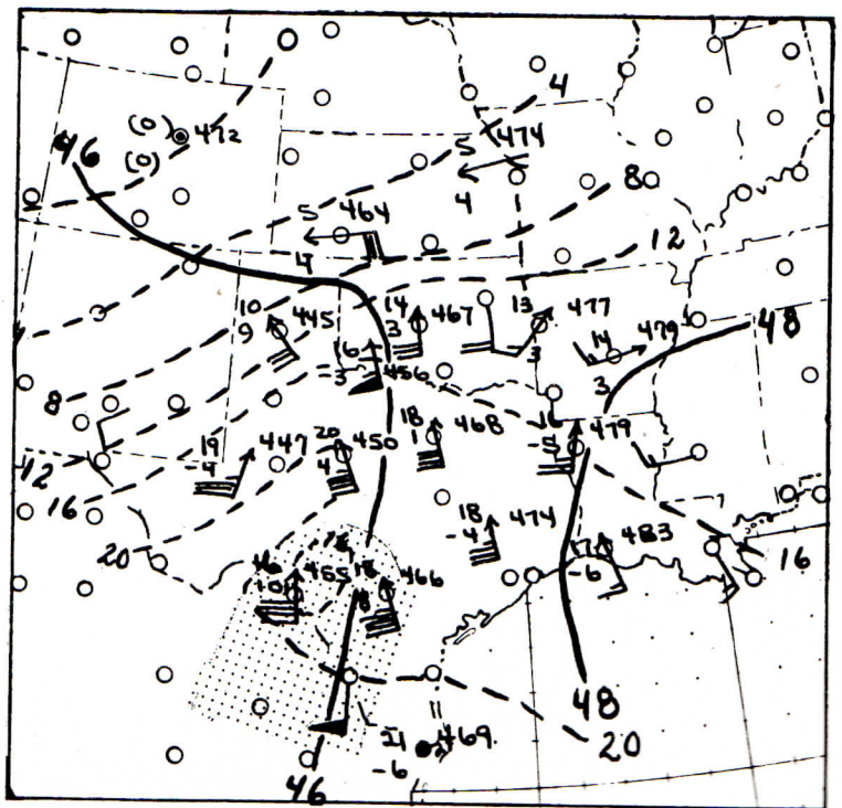
FIGURE 13.—850-millibar chart, 2100 CST, April 1, 1957.
