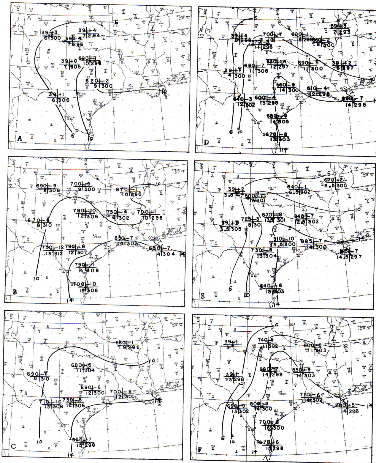
FIGURE 33.—RAOB analysis charts, 1500 cst, April 1, 1957. Level of free convection upper right, average mixing ratio of lower 3,000 feet, upper left on station model, lifted stability index lower left, average mixing ratio of lower 3,000 feet, lower right. Solid lines drawn for values of 6, 10, 14 grams per kilogram mixing ratio. (A) 1500 cst, April 1; (B) 2100 cst, April 1; (C) 0300 cst, April 2; (D) 0900 cst, April 2; (E) 1500 cst, April 2; (F) 2100 cst, April 2.
