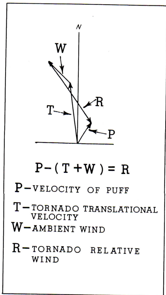
FIGURE 13.—Method of deriving tornado relative wind vector R , from local wind P , ambient wind W , and tornado translational velocity T .
