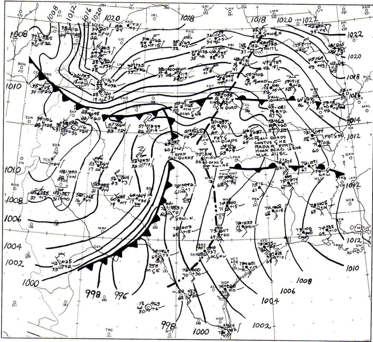
FIGURE 10.—Sectional surface chart, 2130 cst, April 2, 1957.
