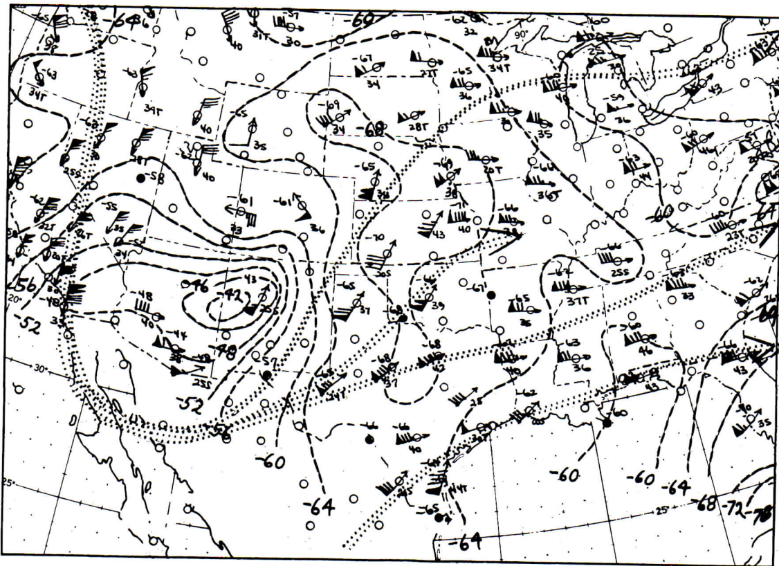
FIGURE 36.—Tropopause and jet chart, 0900 cst, April 2, 1957.
