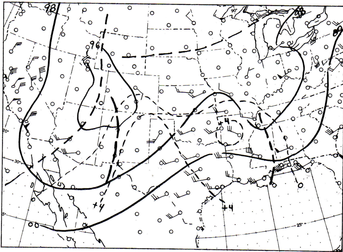
FIGURE 19.—700-millibar chart, 1500 CST, April 1, 1957.
