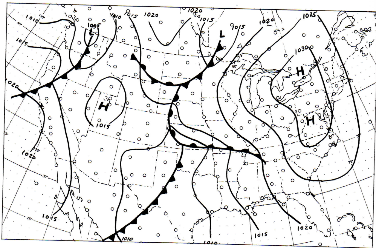
FIGURE 2.—Surface pressure map, 0630 cst, March 31, 1957.
