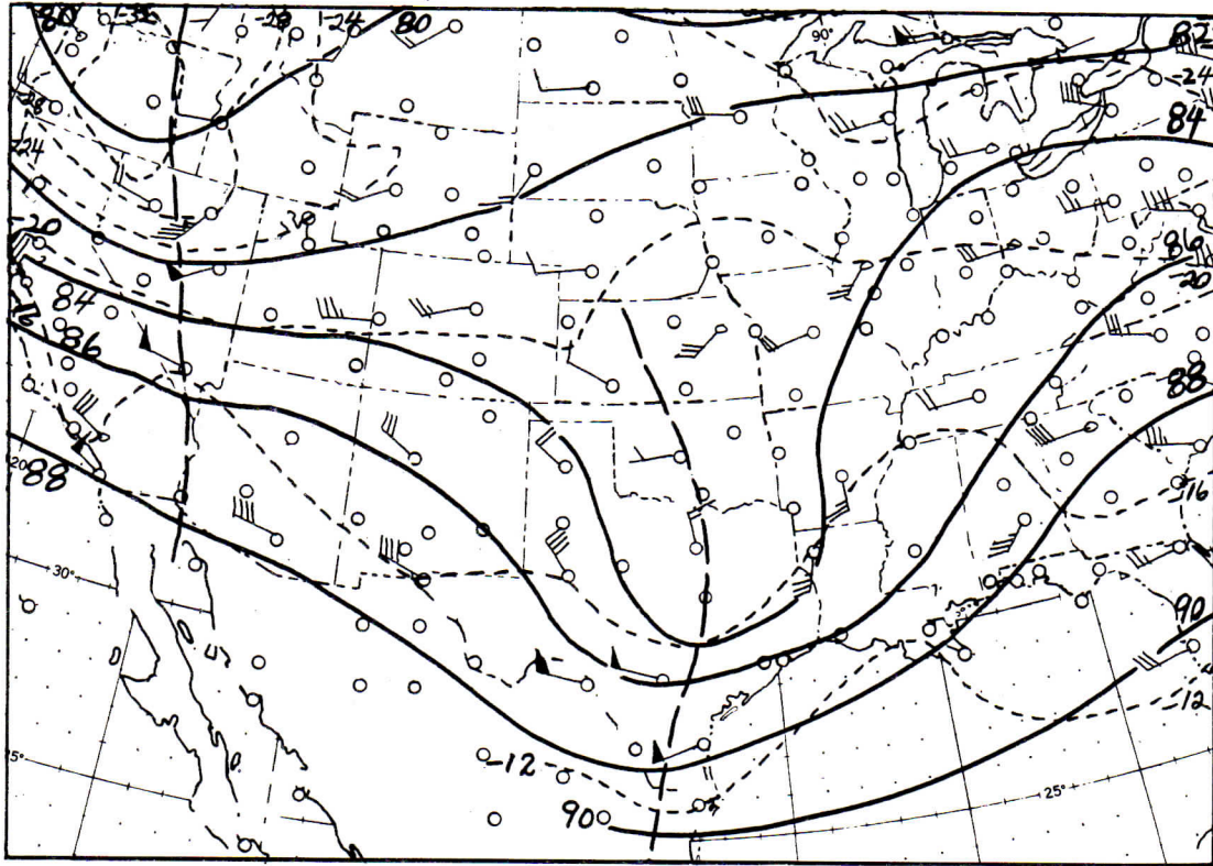
FIGURE 26.—500 millibar chart, 2100 CST, March 31, 1957.
