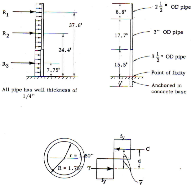
FIGURE 8.—Dimensions of flagpole (above), and stress distribution in pole, item no. VIII.
