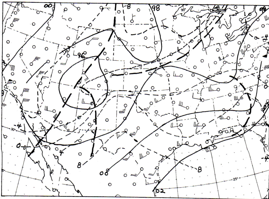
FIGURE 20.—700-millibar chart, 2100 CST, April 1, 1957.
