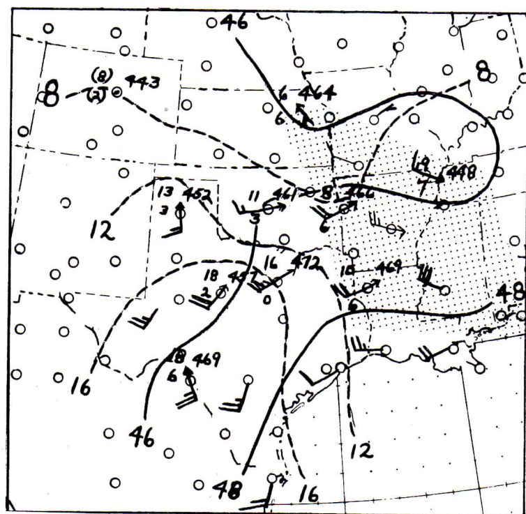
FIGURE 12.—850-millibar chart, 1500 CST, April 1, 1957.
