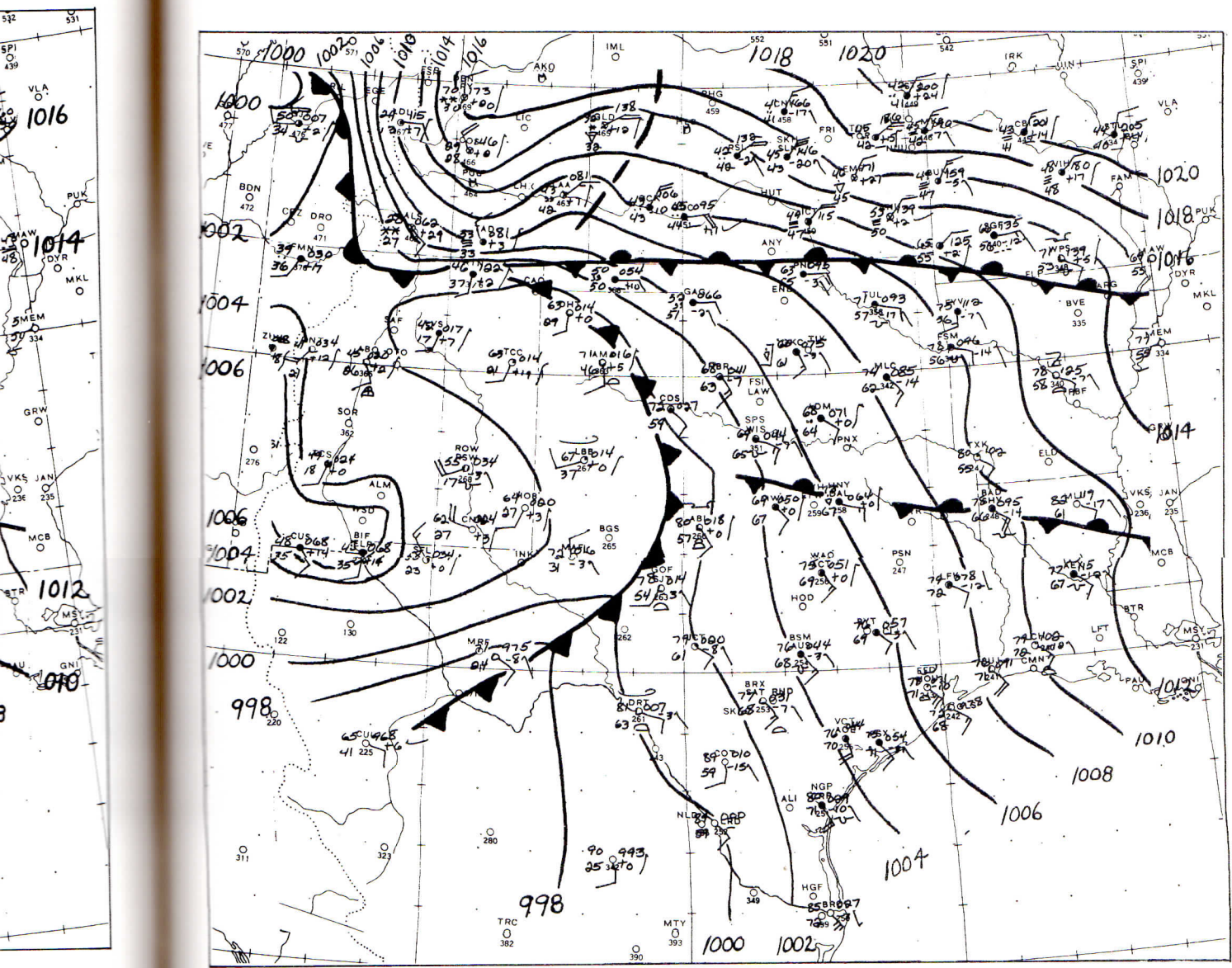
FIGURE 7.—Sectional surface chart, 1230 cst, April 2, 1957.
