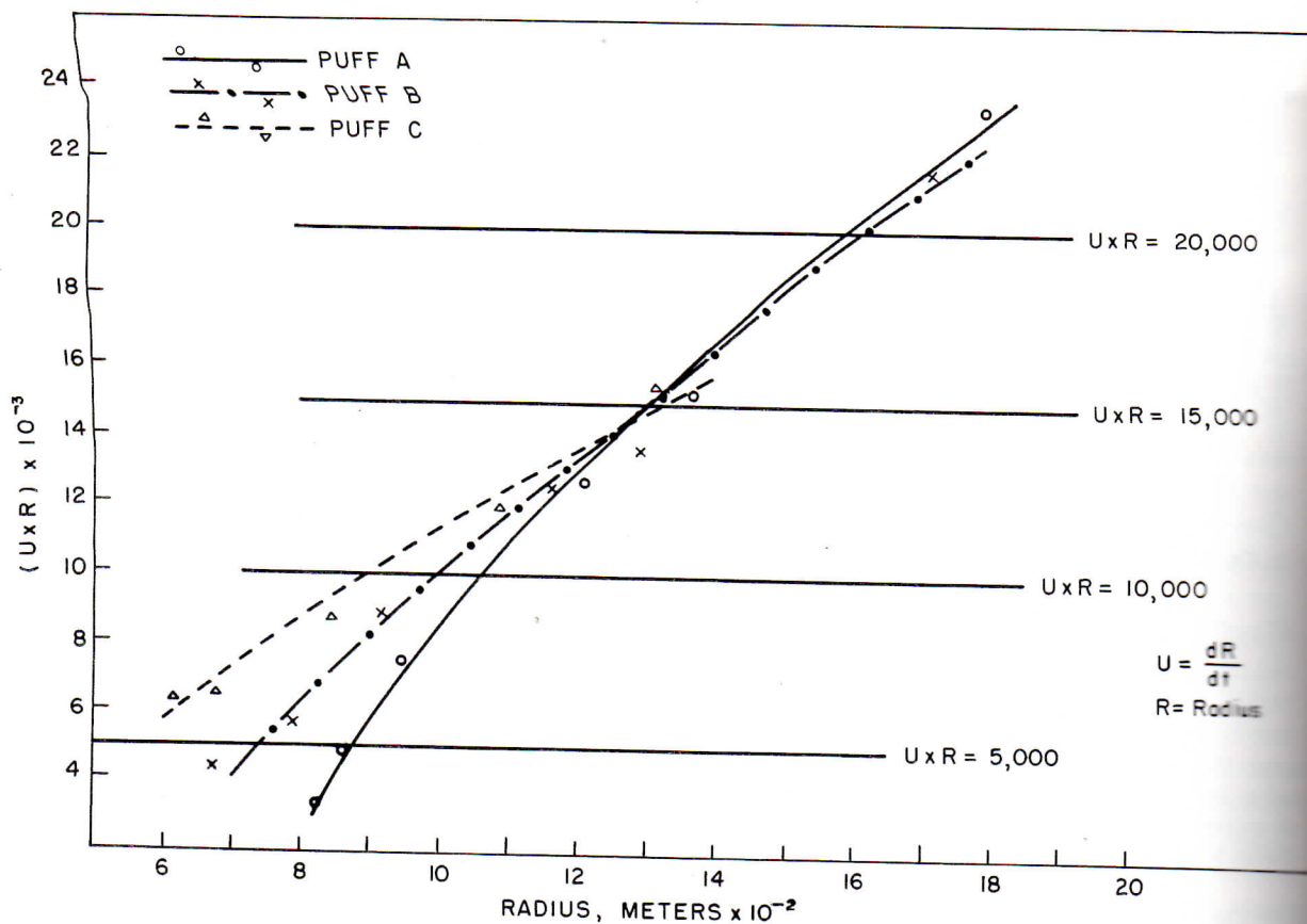
FIGURE 19.—Variations of radial component wind times radius ( U \times R ) with R , for the tornado-wind. Families of curves with (U \times R) = \text{constant} , denoting nonconvergence, also are shown. The curves for the Dallas tornado indicate convergence for the region investigated.
