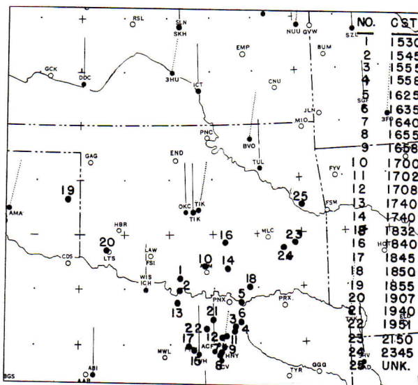
FIGURE 1.—Location and time (cstr) of tornadoes in Texas and Oklahoma, April 2, 1957.
