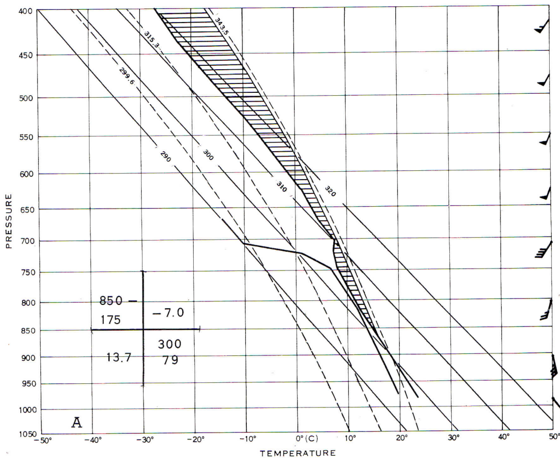
FIGURE 5.—Carswell AFB sounding for 1930 cst April 2, 1957. The inversion has descended and the upper-level moisture has disappeared. A large positive energy area, extending to the tropopause, still exists.
