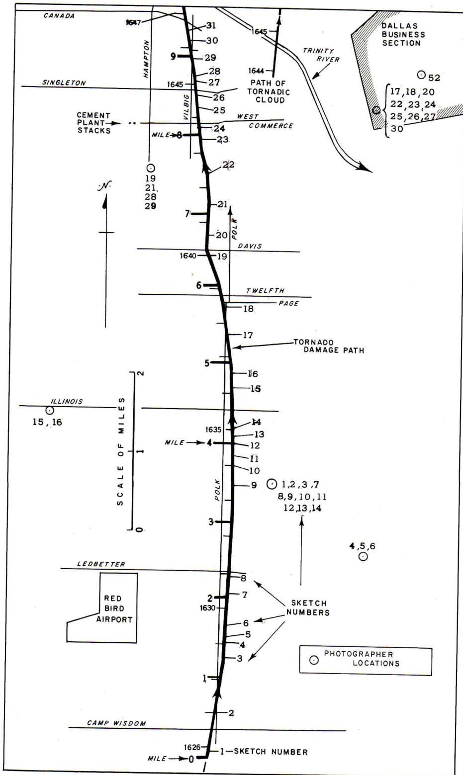
FIGURE 1.—South section.—Dallas tornado damage path and path of tornadic cloud. To the left of the damage path is marked the mileage along the damage path and the minute-by-minute locations of the tornado. To the right of the damage path are the locations of the tornado at the times of the numbered sketches of figure 2. The photographer-locations for the various sketches are shown by the circled dots.
