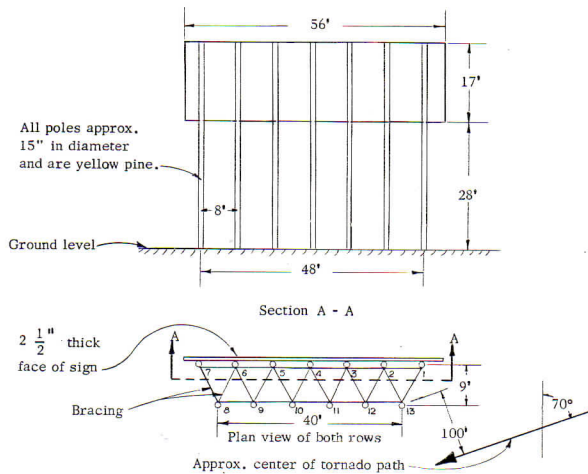
FIGURE 5.—End elevation of sign (above), front view (center), and plan view of sign, item no. V.
